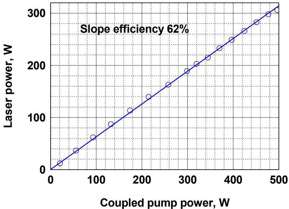
Figure 4 - Laser slope efficiency
