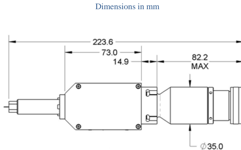
Figure 3 Output Device of NUQQ-1064-NA-0010-CZ, NUQA-1064-NA-0020-CZ, and NUQA-1064-NA-0030-CZ
